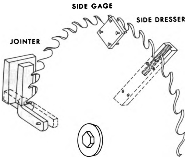
2 TOOLS FOR ALINING SAW
